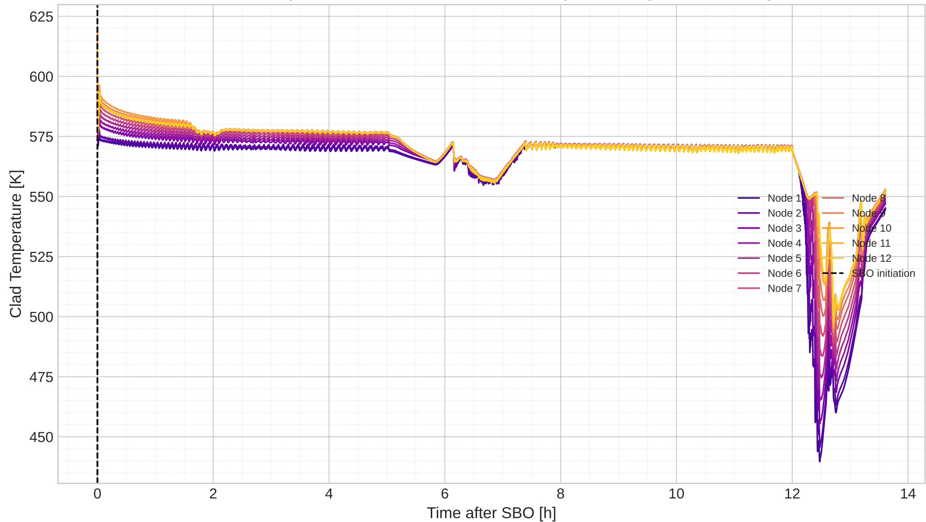
No SG Depressurization - Clad Surface Temperatures (all axial nodes)
